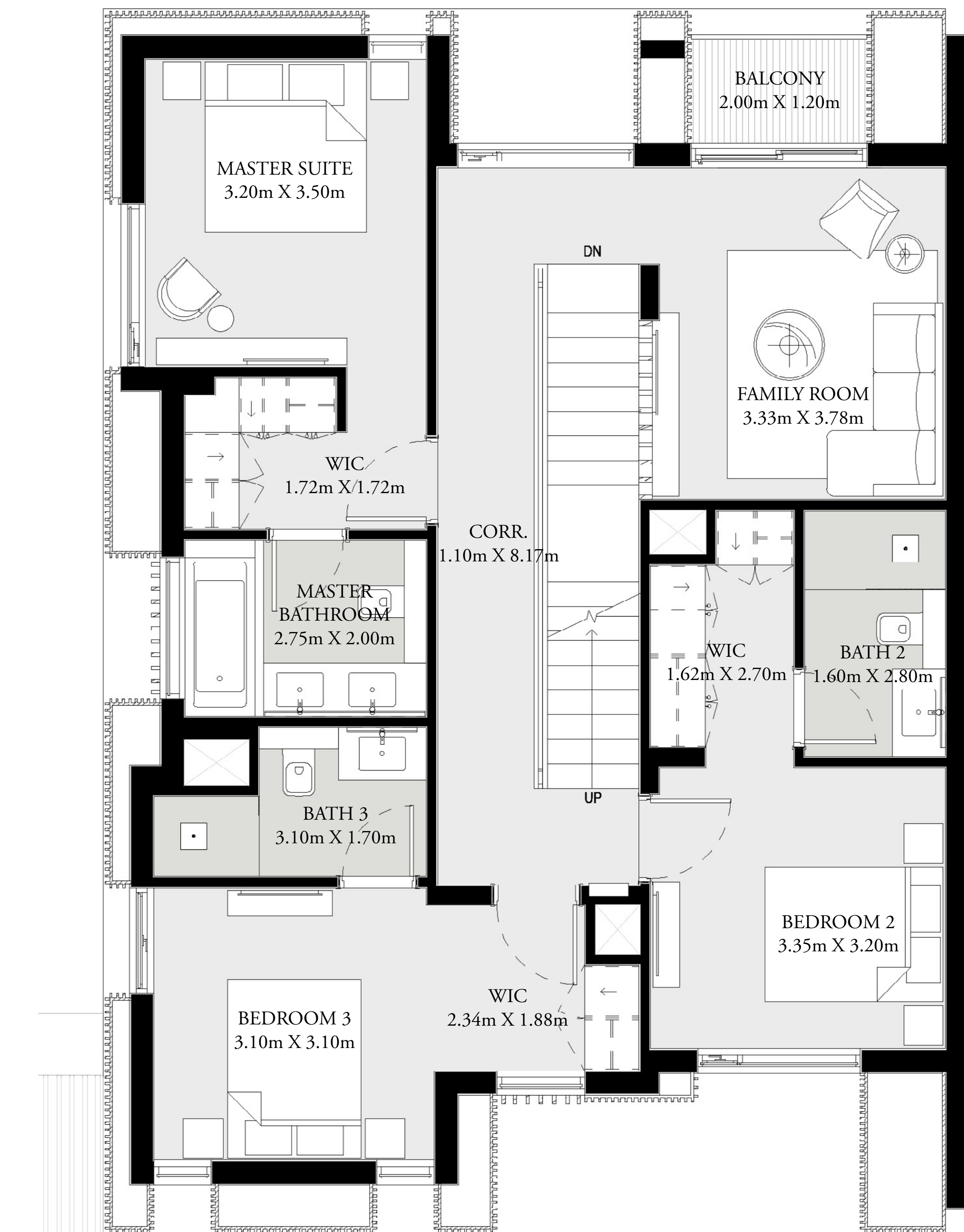
FIRST FLOOR
