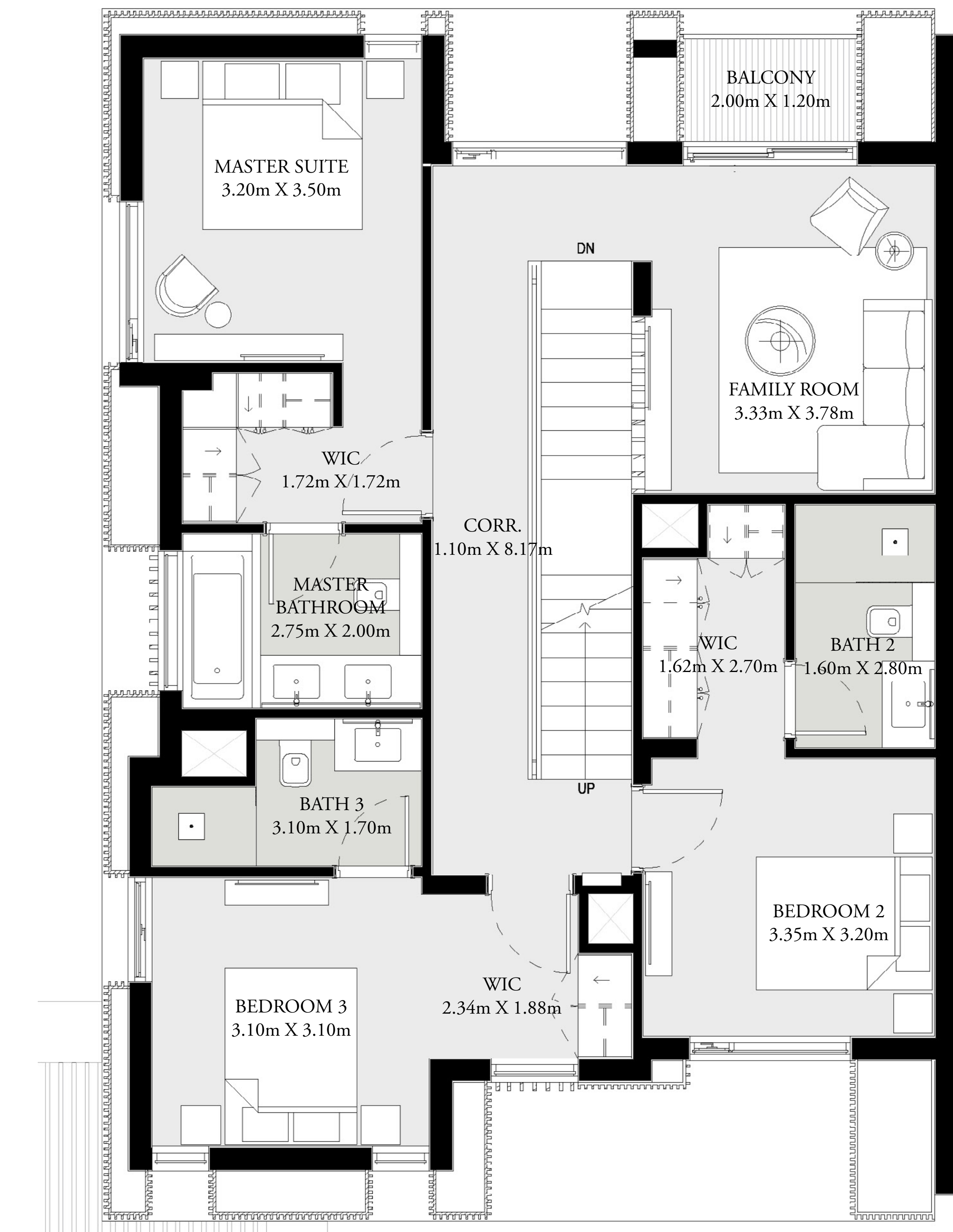
FIRST FLOOR
