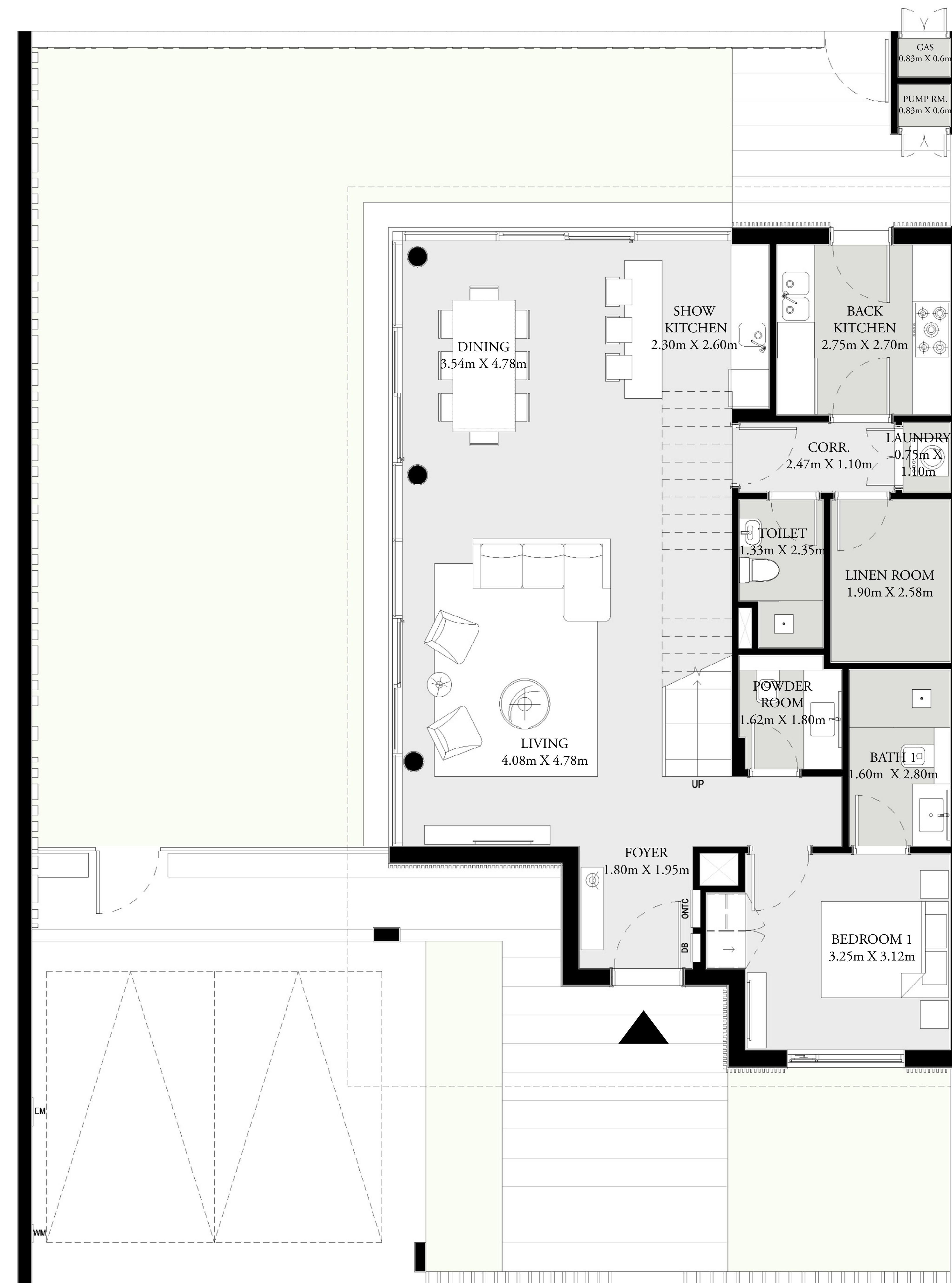
GROUND FLOOR
